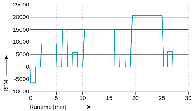
Endurance test 28-minute speed cycle repeated for the full test duration.
