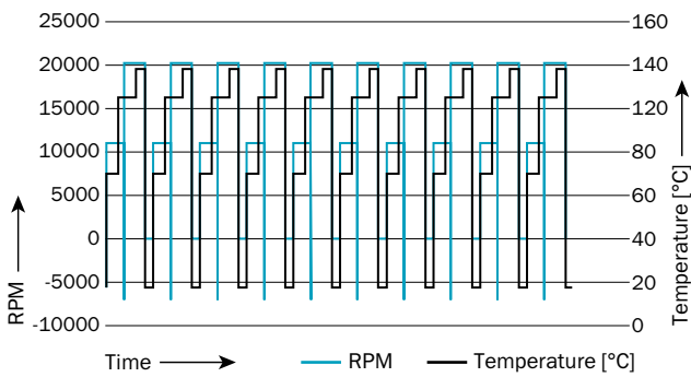
Extreme speed and temperature conditions in the high-speed test.
