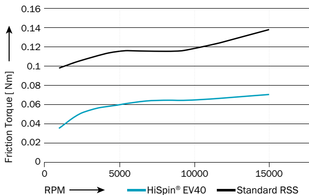
Torque loss measurements comparing the Stefa® HiSpin® EV40 with a standard radial shaft seal.
